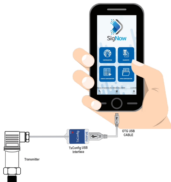
Figure 9 – OTG Cable
