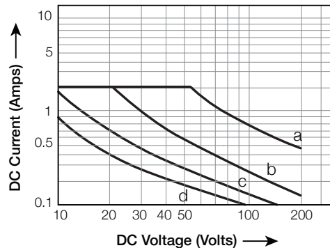
Maximum dc inductive load breaking capacity
